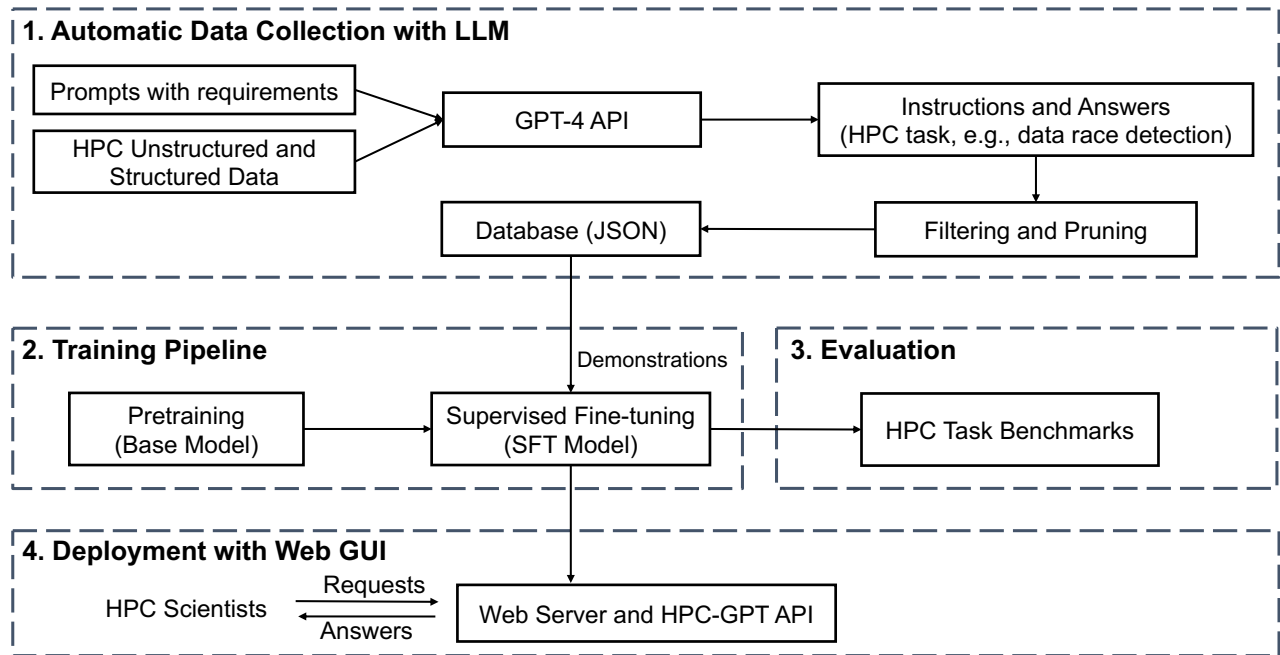
Figure 1: HPC-GPT Architecture.
